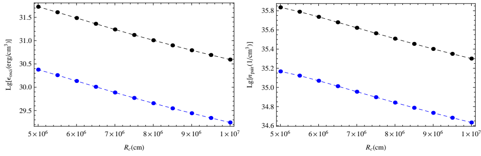
Figure C.4.: The energy (left) and number (right) densities of electron-positron pairs at selected values of collapsing radii R_c for M = 10M_\odot and N_p/N_B \approx 1/38 (upper); 1/380 (lower). We select R_c^{\text{max}} \sim 10^7 \text{cm} so that \bar{n}_B \sim n_{\text{nucl}} .
