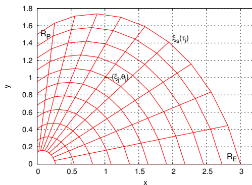
Figure 0.7: Numerical grid used in simulations.
