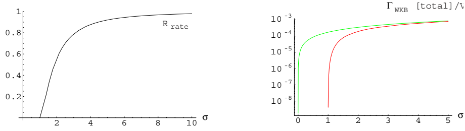
Figure 6.3: Left: Ratio R_{\text{rate}} defined in Eq. (6.3.24) is plotted as function of \sigma_s in the left figure. Right: Number of pairs created in slab of Compton width per area and time as functions of \sigma_s . Upper curve is for the constant field (6.3.2), lower for the Sauter field (6.3.15)). Both plots are for E_0 = E_c and \sigma_s = \ell/\lambda_C .
