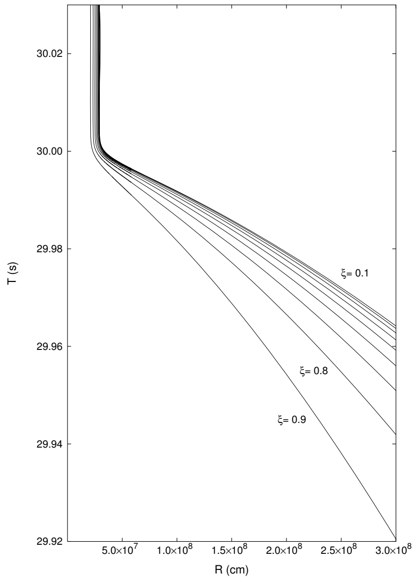
Figure 8.8: Collapse curves in the plane (T, R) for M = 20M_{\odot} and for different values of the parameter \zeta . The asymptotic behavior is the clear manifestation of general relativistic effects as the horizon of the black hole is approached. Details in [405].
