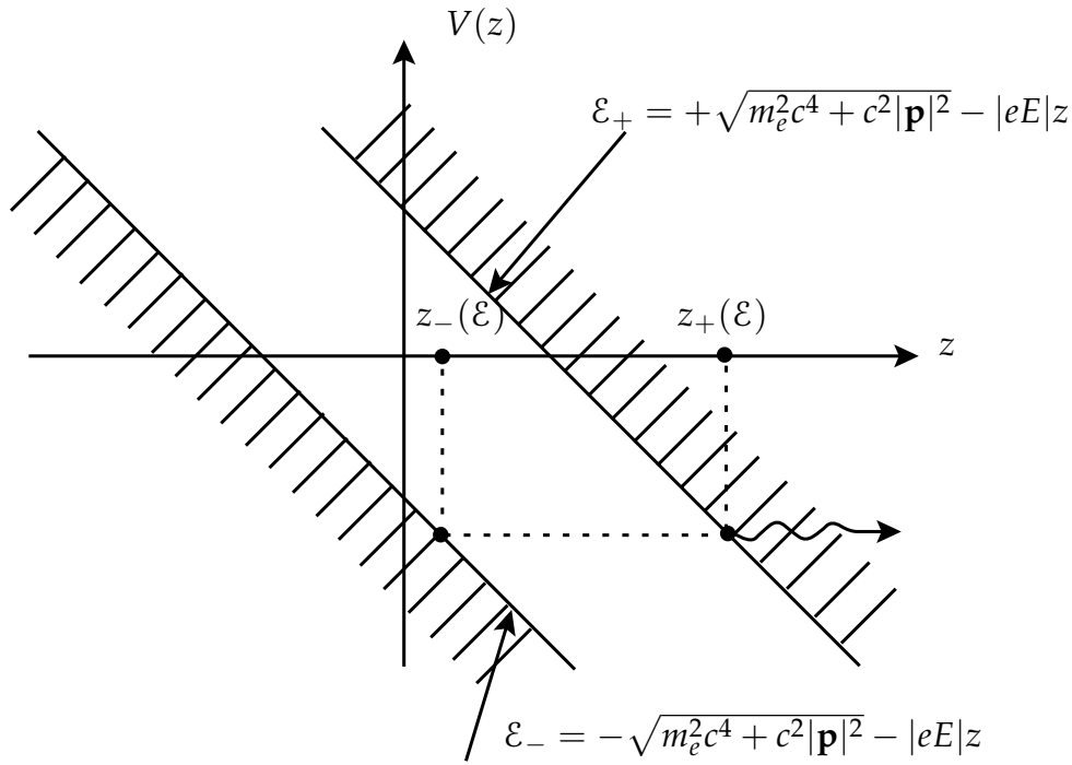
Figure 3.4: Energy-spectra \mathcal{E}_{\pm} with an external electric field \mathbf{E} along \hat{z} -direction (for -\ell < z < \ell and \ell \gg 1 ). Crossing energy-levels appear, indicated by a dashed line between two continuum energy-spectra \mathcal{E}_{-} and \mathcal{E}_{+} . The turning points z_{\pm}(\mathcal{E}) for the crossing energy-levels \mathcal{E} of Eq. (3.5.5) are marked. This implies that virtual electrons at these crossing energy-levels in the negative energy-spectrum can quantum-mechanically tunnel toward infinity [ z \gg z_{+}(\mathcal{E}) ] as real electrons; empty states left over in the negative energy-spectrum represent real positrons. This is how quantum tunneling produces pairs of electrons and positrons.
