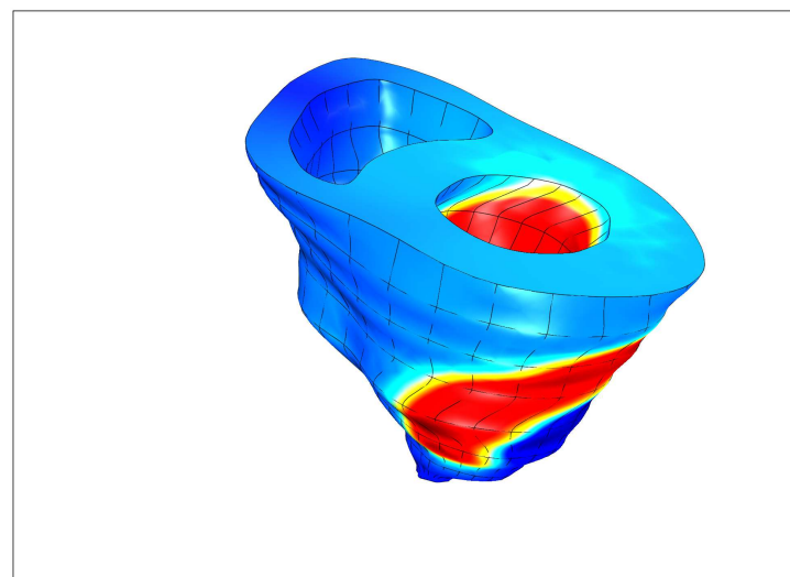
Figure 0.4: 3D spiral waves iso-voltage lines embedded in a mechanically deformed domain.
