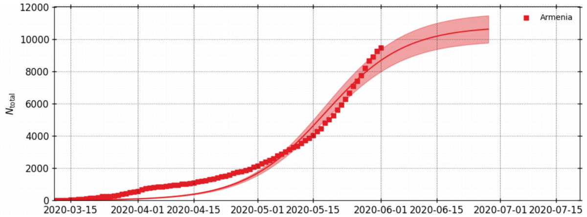
Total number of confirmed Covid-19 cases: 02.06.2020
